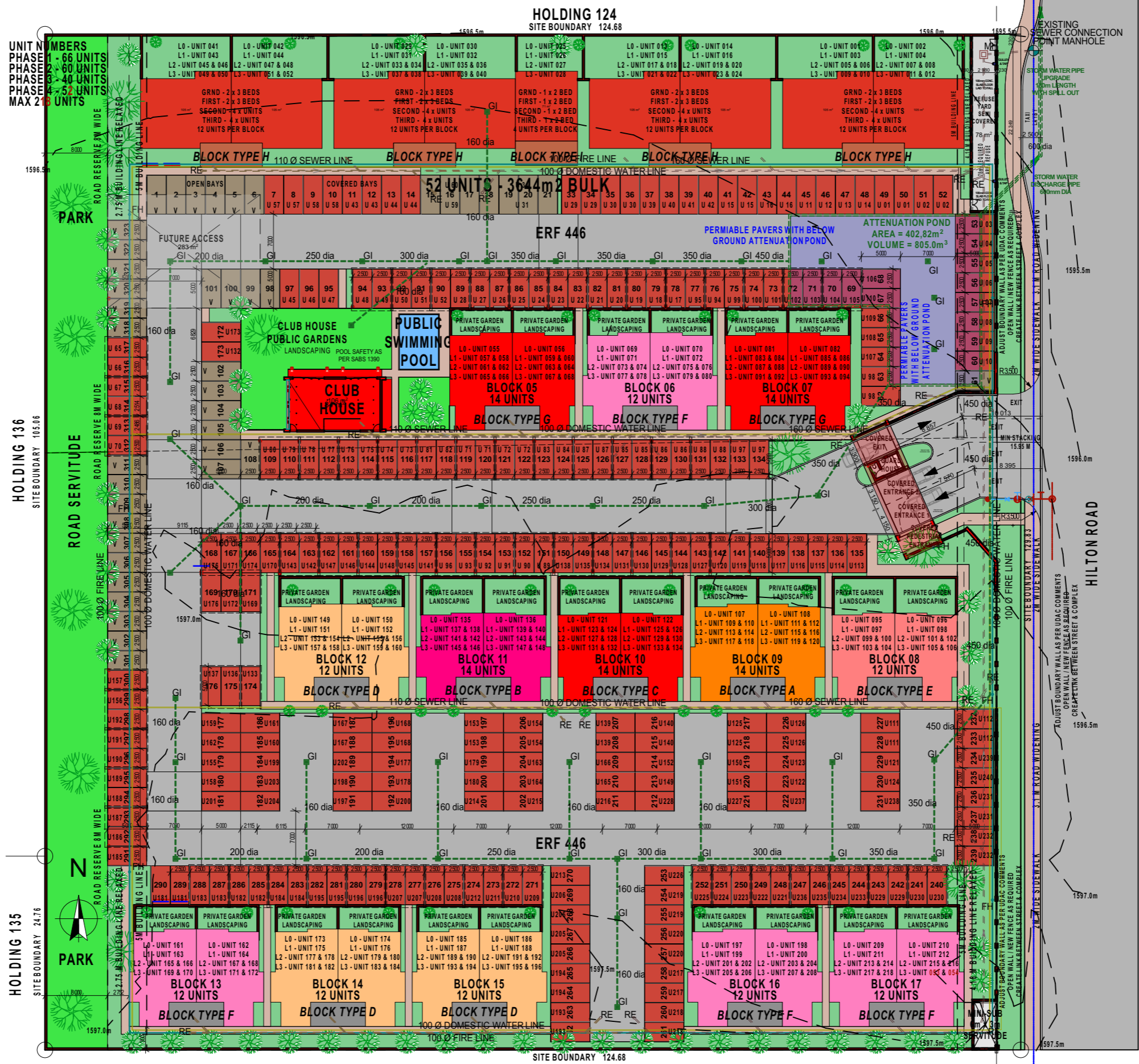
SITE PLAN SCALE 1:550
